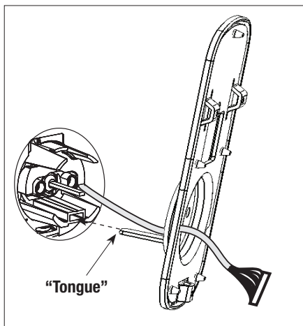
Figure 4B
